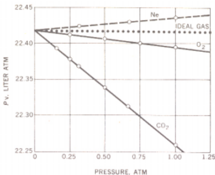
FIGURE 1-5 Accurate data for the product PV for 1 mol of the gas as a function of pressure at 0^\circ\text{C} . (Adapted from L. P. Hammett, "Introduction to the Study of Physical Chemistry," Copyright 1952 by McGraw-Hill, Inc. Used by permission of McGraw-Hill Book Company.)
